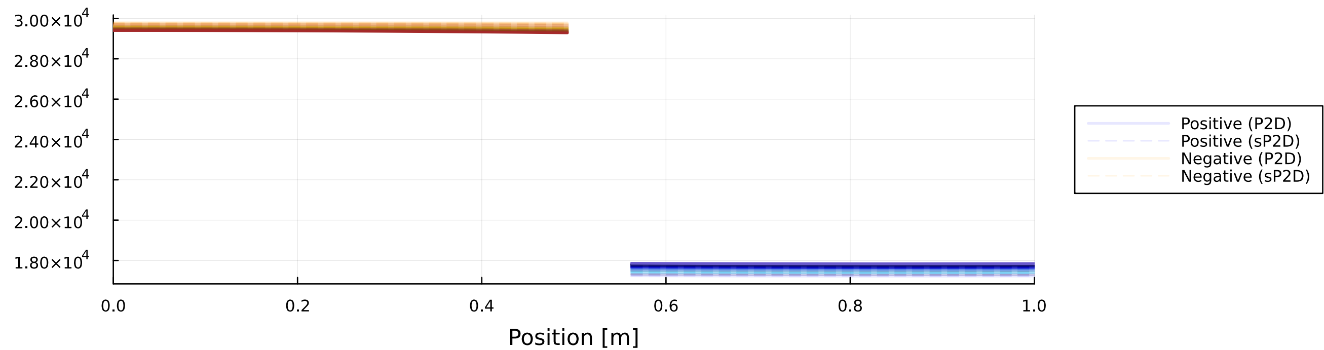
Electrode Stress Distribution (P2D & sP2D) - High Frequency Pulse
